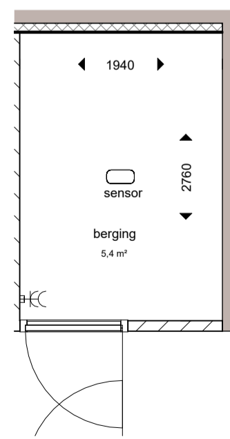
berging
