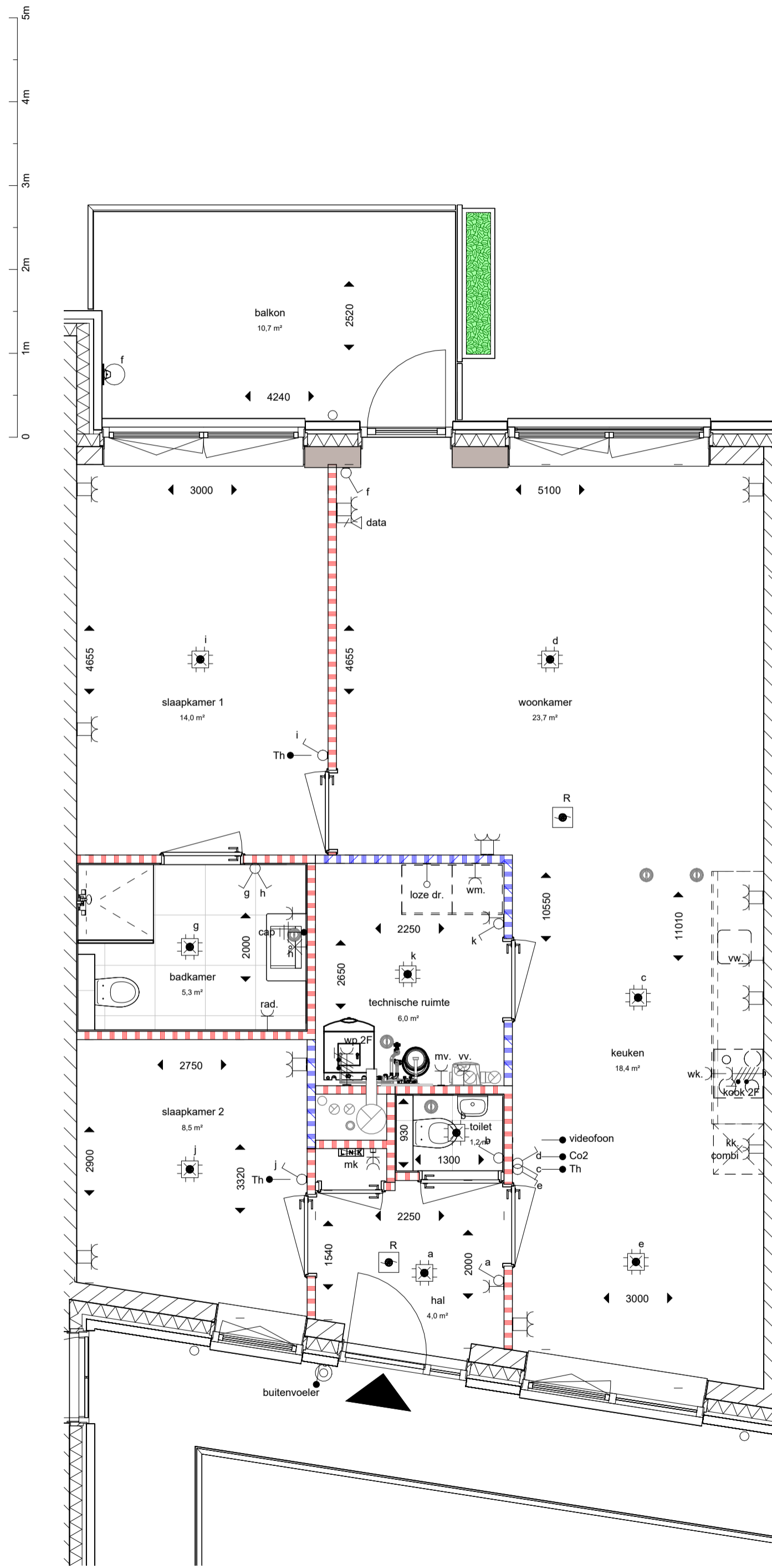
bnr 21 - type (Central Park)
