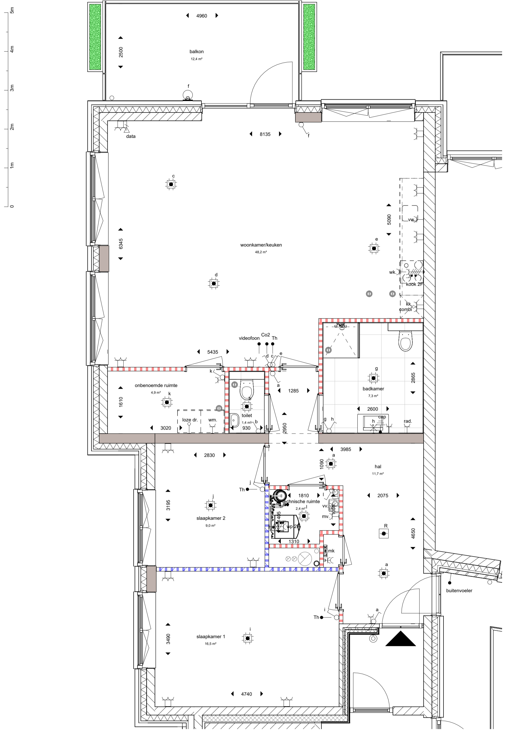
bnr 29 - type (Kensington Park)
