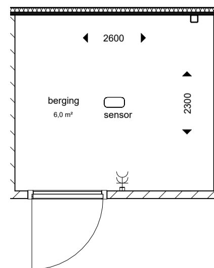
berging
