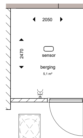
berging
