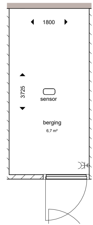
berging 1:50
