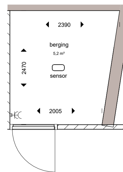
berging
