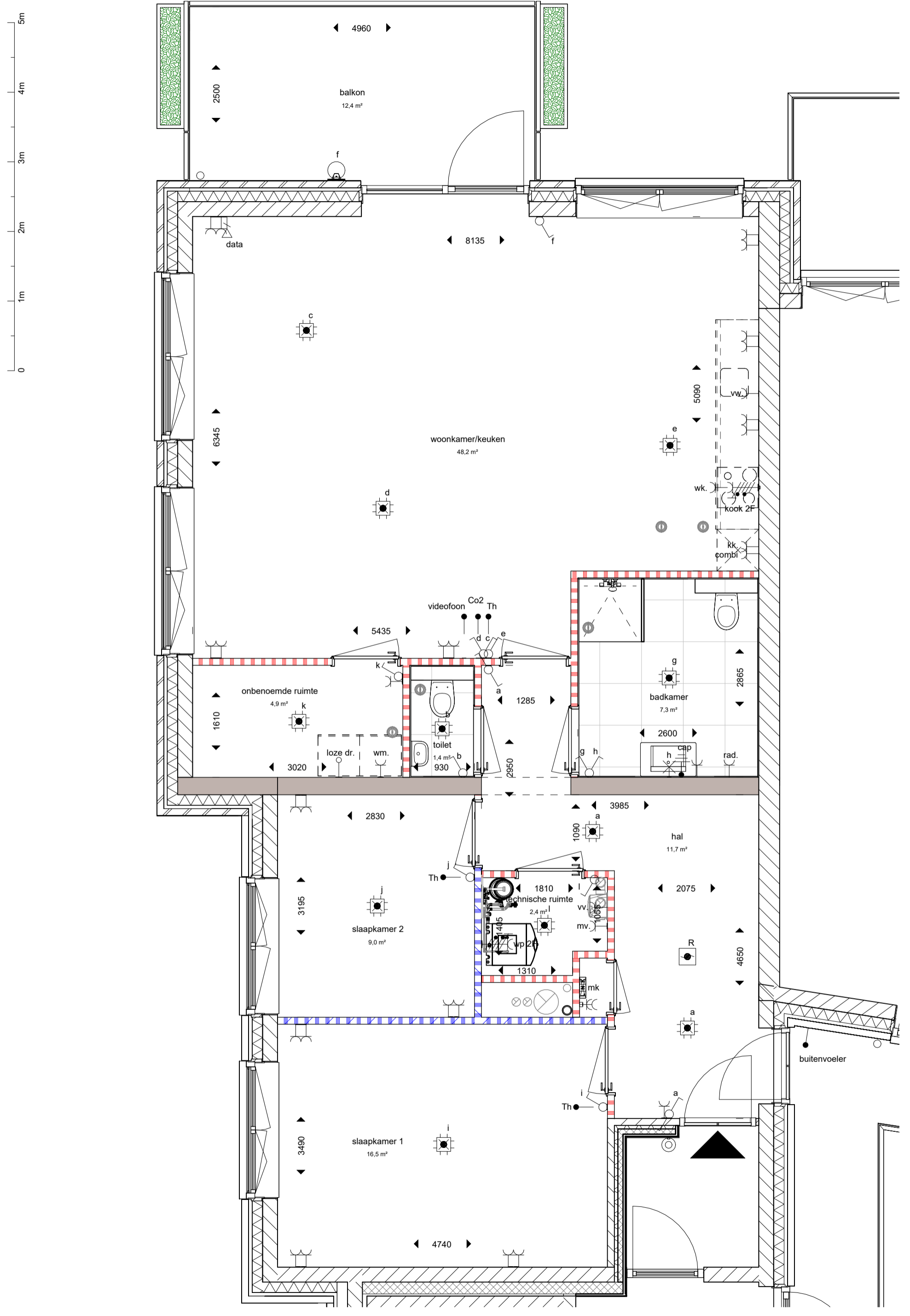
bnr 35 - type (Kensington Park)
