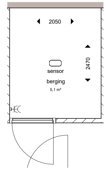
berging
