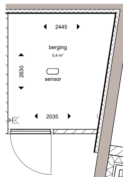
berging
