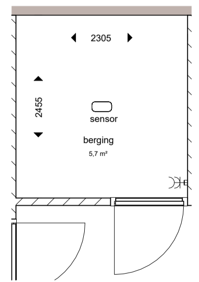
berging 1:50
