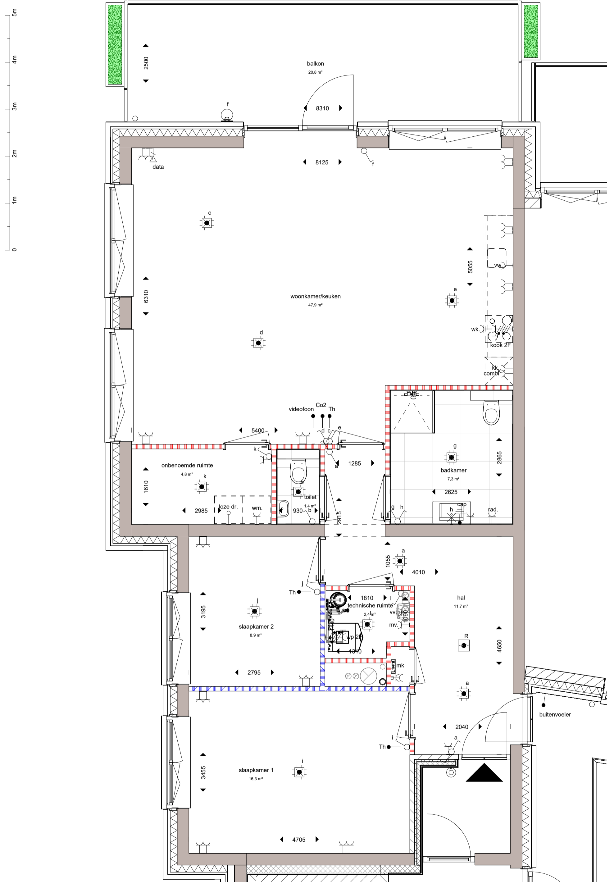
bnr 14 - type (Kensington Park)
