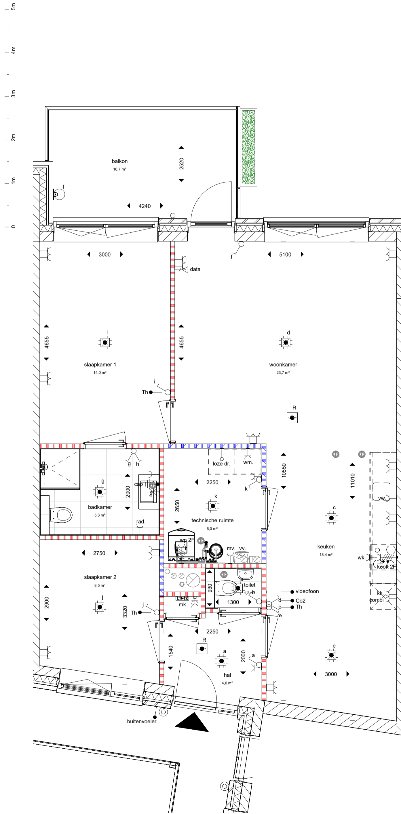
bnr 32 - type (Central Park)
